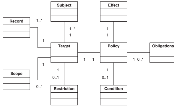
Fig. 6. An Access Control Language
