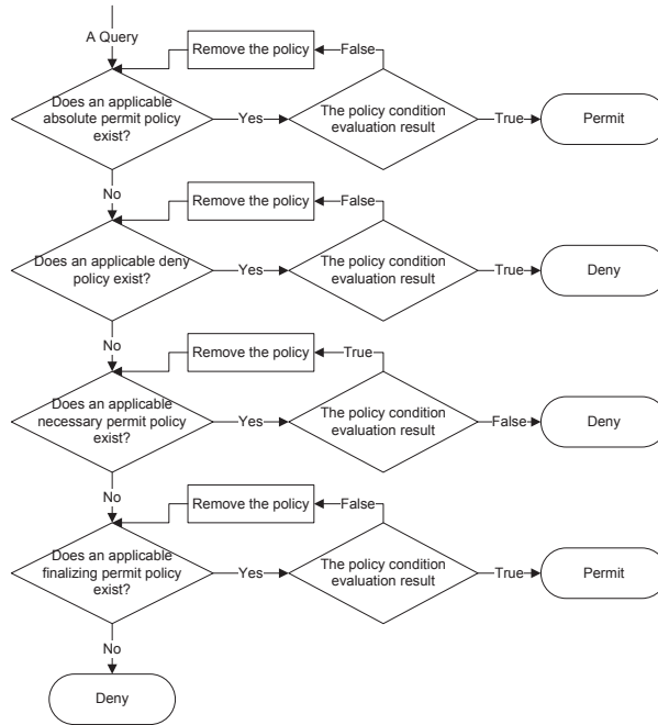
Fig. 7. Policy Evaluation Flow
