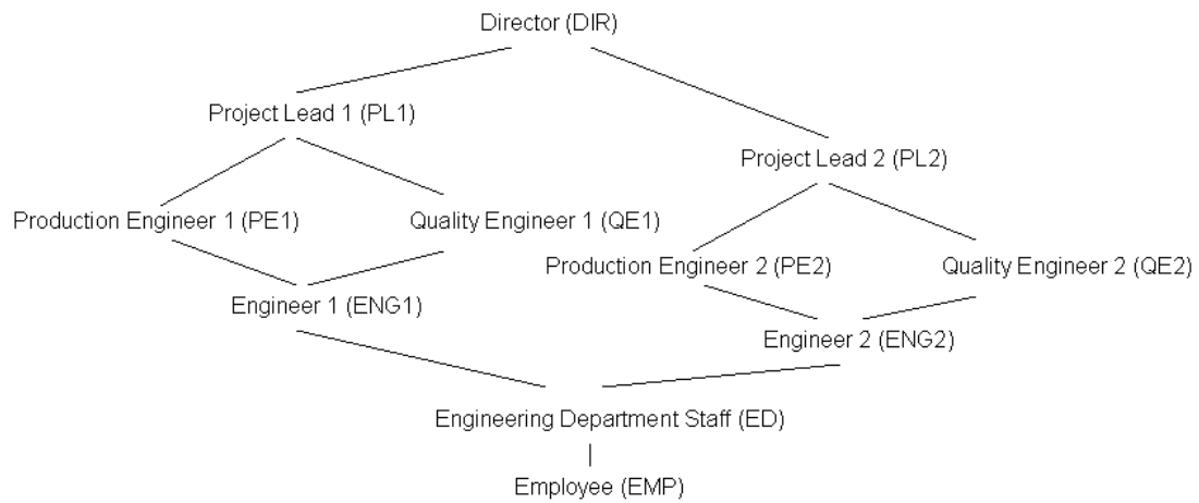
(a) An example of regular role hierarchy
