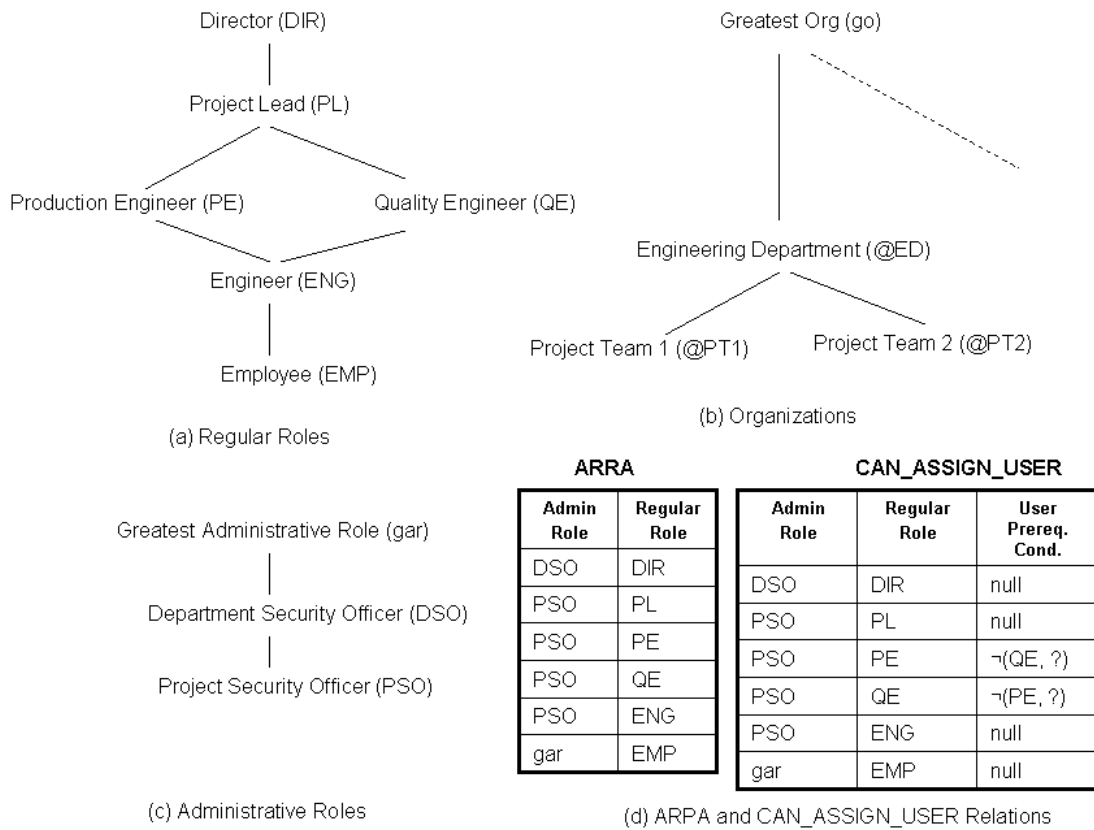
Figure 7. Role and organization hierarchies using administrative ROBAC
